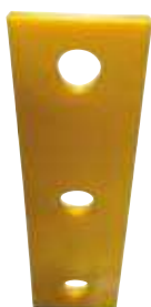
Front plate. Hardwearing PE. 710 x 210 x 35 mm Weight: 4,5 kg
